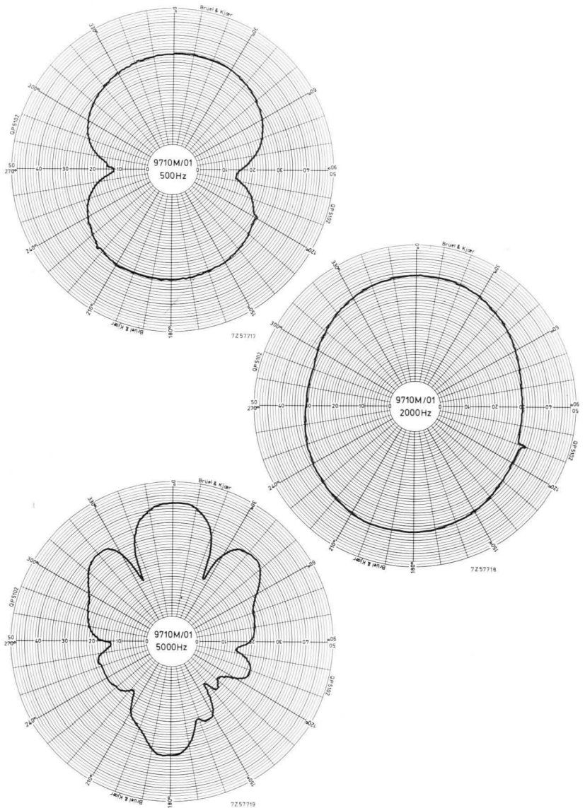
Fig. 5. The polar response curves of a typical high quality full-range speaker at different frequencies. Note the fall in output at 90^\circ and 270^\circ on the 500 Hz curve due to acoustic short-circuiting.
