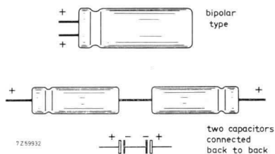
Fig. A.2. Showing how two electrolytic capacitors can be connected to produce the equivalent of a bipolar type.
