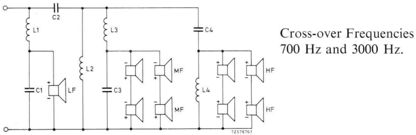
Cross-over Filter Network as for System 17 showing the squawkers in series/parallel and the tweeters in series/parallel.
