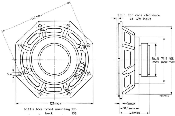
5" Standard Loudspeaker
