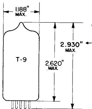
GLASS BULB BASE E9-68 JEDEC OUTLINE 9-70
