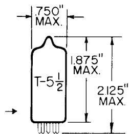
GLASS BULB MINIATURE PUTTON 7 PIN BASE E7-1 OUTLINE DRAWING JEDEC 5-7
