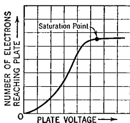
Fig. 5—Current characteristic of diode tube.
