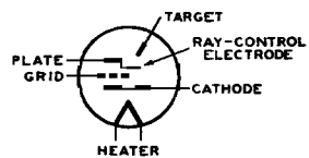
ELECTRON-RAY TUBE
