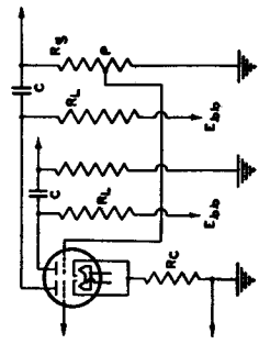
TWIN-TRIODE DIAGRAM WITH LEGEND
