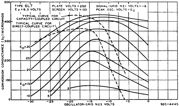
AVERAGE CHARACTERISTICS FOR TYPE 6L7
