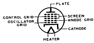
PENTAGRID CONVERTER
