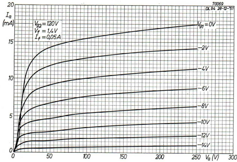
Fig. 67. Anode current plotted against anode voltage for V_{g2} = 120 V and V_f = 1.4 V , I_f = 0.05 A .
