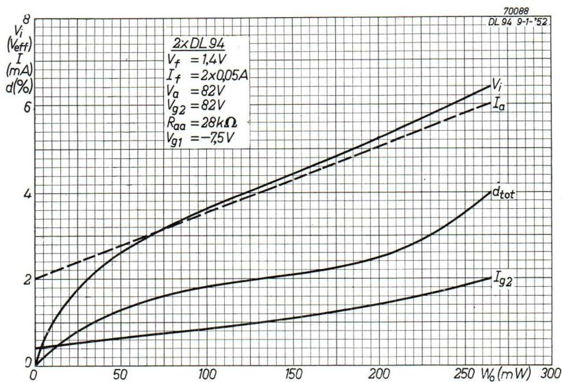
Fig. 86. Performance of two DL 94 tubes in push-pull class B for V_b = 90V and V_f = 1.4V , I_f = 2 \times 0.05A (parallel arrangement of one filament section of each tube).
