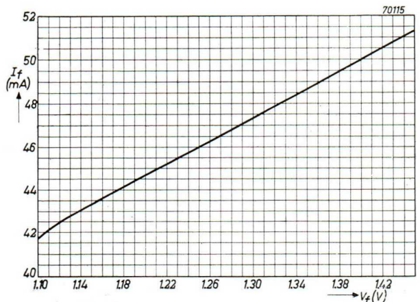
Fig. 114. Filament current plotted against filament voltage for a 50 mA miniature battery tube.
