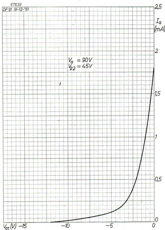
Fig. 23. Anode current plotted against control-grid voltage for V_{g2} = 45 \text{ V} and V_a = 90 \text{ V} .
