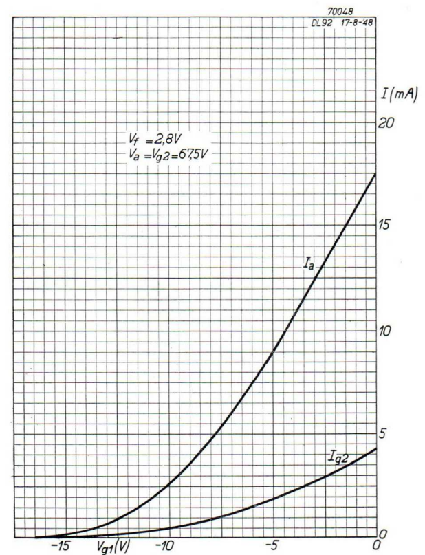
Fig. 45. Anode current and screen-grid current plotted against the control-grid voltage for V_a = V_{g2} = 67.5 V when the two filament sections are connected in series ( V_f = 2.8 V and I_f = 0.05 A).
