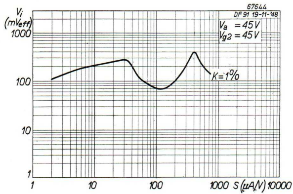
Fig. 28. Input signal plotted against the mutual conductance for a cross modulation of 1%, for V_a = V_{g2} = 45\text{ V} .
