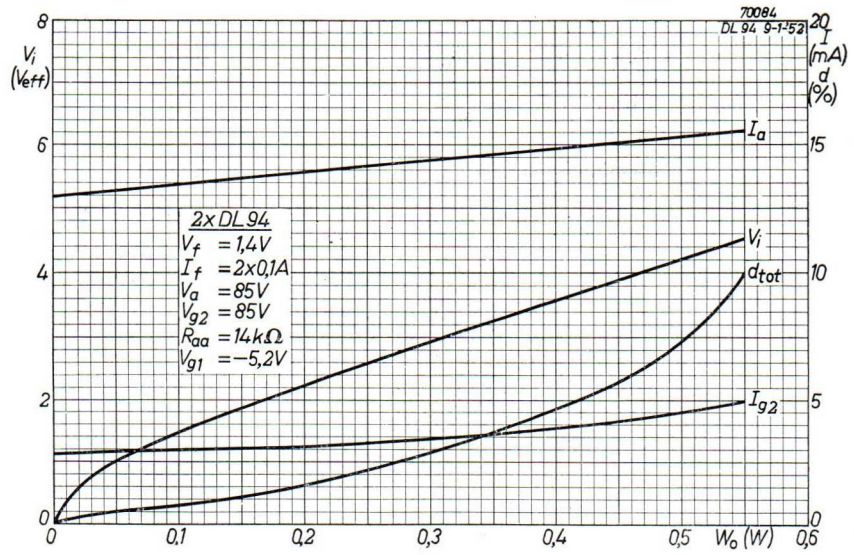
Fig. 82. Performance of two DL 94 tubes in push-pull class A for V_b = 90 V and V_f = 1.4 V, I_f = 2 \times 0.1 A (all filament sections in parallel).
