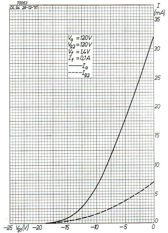
Fig. 61. Anode current and screen-grid current plotted against the control-grid voltage for V_a = V_{g2} = 120 V and V_f = 1.4 V, I_f = 0.1 A.
