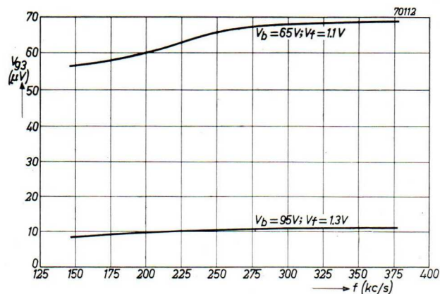
Fig. 111. Sensitivity for the long-wave range.
