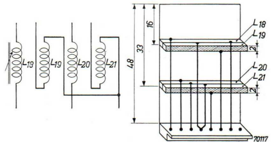
Fig. 116. Development of the oscillator coil combination for the ranges M.W. and L.W.
