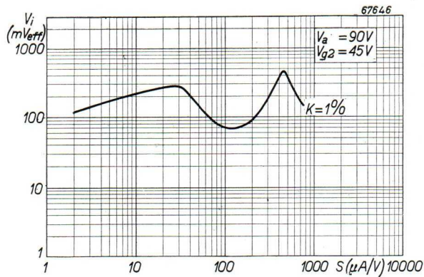
Fig. 30. Input signal plotted against the mutual conductance for a cross modulation of 1%, for V_a = 90\text{ V} and V_{g2} = 45\text{ V} .
