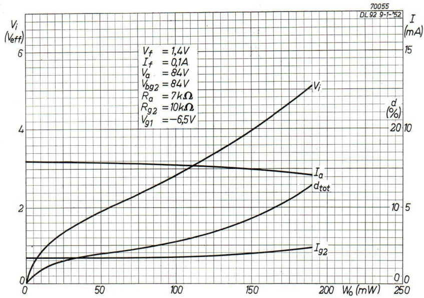
Fig. 52. Anode current, screen-grid current, input voltage and total distortion plotted against the output for V_b = 90V , and V_f = 1.4V , I_f = 0.1A .
