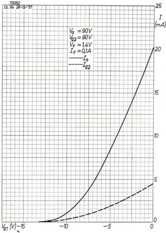
Fig. 60. Anode current and screen-grid current plotted against the control-grid voltage for V_a = V_{g2} = 90 V and V_f = 1.4 , I_f = 0.1 A (two filament sections in parallel).
