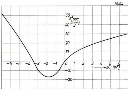
Fig. 103. Pulling of the oscillator frequency plotted against the capacitance variation of the input circuit for an oscillator frequency of 20 Mc/s.
