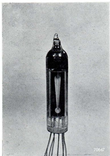
Fig. 95. The tuning indicator DM 70.
