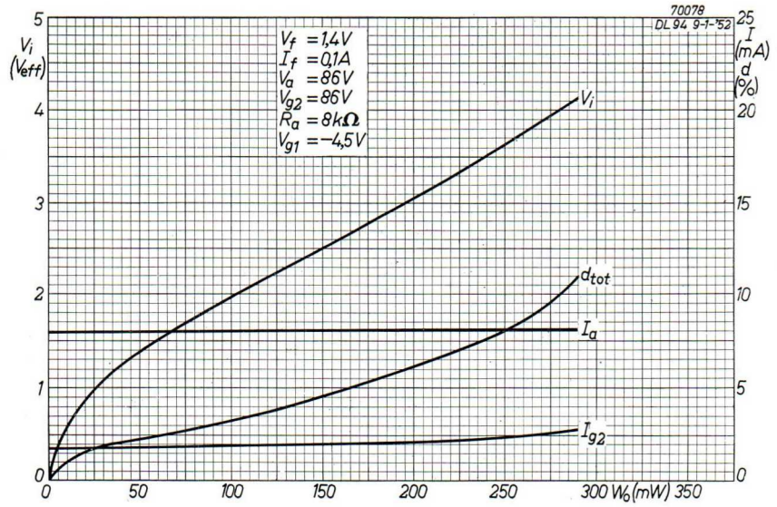
Fig. 76. Performance of one DL 94 tube in class A for V_b = 90 V and V_f = 1.4 V, I_f = 0.1 A (two filament sections in parallel).
