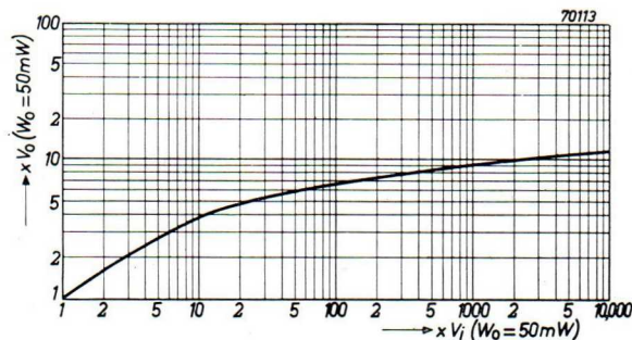
Fig. 112. The A.G.C. curve measured in the medium-wave range.
