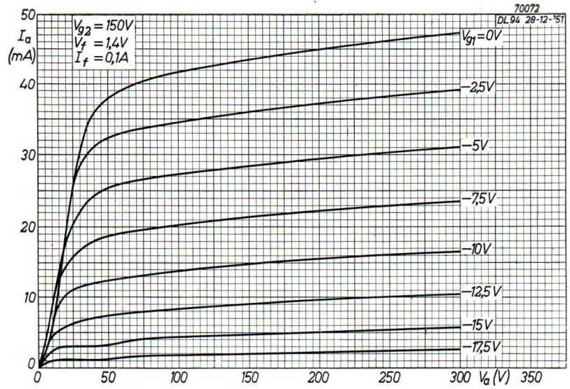
Fig. 70. Anode current plotted against anode voltage for V_{g2} = 150 V and V_f = 1.4 V, I_f = 0.1 A.
