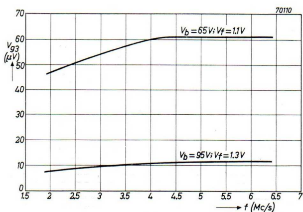
Fig. 109. Sensitivity for the range S.W. 2.
