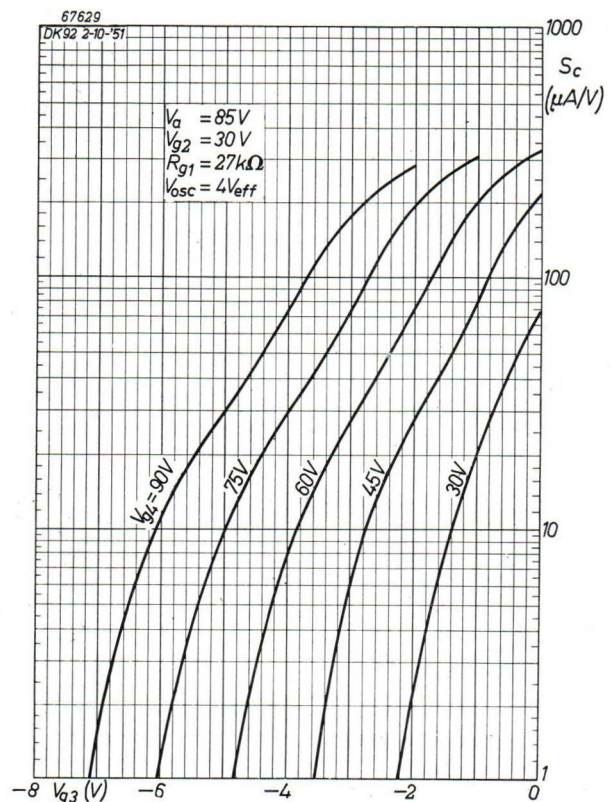
Fig. 12. Conversion conductance as a function of the third-grid voltage with the screen-grid voltage as parameter, for V_a = 85 V.
