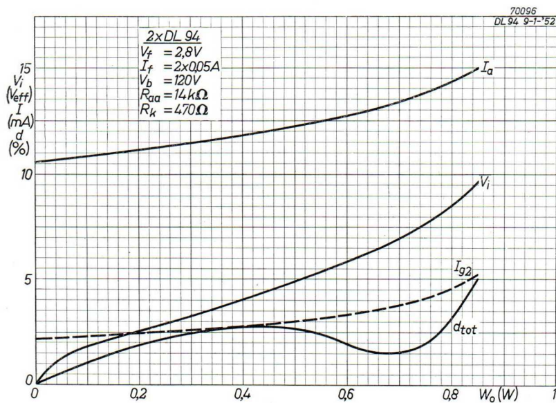
Fig. 94. Performance of two DL 94 tubes in push-pull class AB for V_b = 120 V and V_f = 2.8 V, I_f = 2 \times 0.05 A (filament sections of each tube in series, filaments of the two tubes in parallel).
