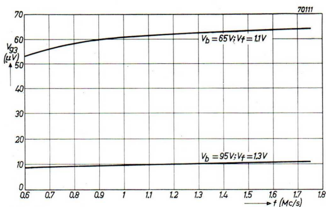
Fig. 110. Sensitivity for the medium-wave range.
