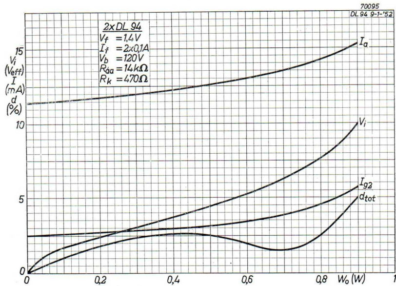
Fig. 93. Performance of two DL 94 tubes in push-pull class AB for V_b = 120 V and V_f = 1.4 V, I_f = 2 \times 0.1 A (all filament sections in parallel).
