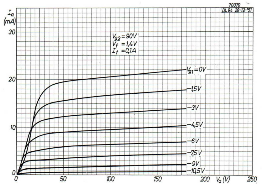
Fig. 68. Anode current plotted against anode voltage for V_{g2} = 90 V and V_f = 1.4 V , I_f = 0.1 A .
