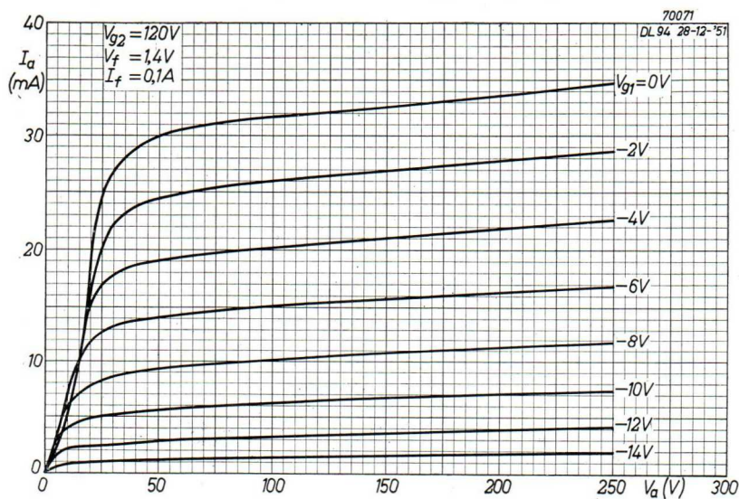
Fig. 69. Anode current plotted against anode voltage for V_{g2} = 120 V and V_f = 1.4 V , I_f = 0.1 A .
