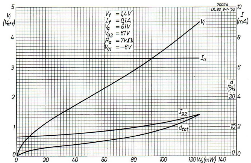
Fig. 51. Anode current, screen-grid current, input voltage and distortion plotted against the output for V_b = 67.5 V and V_f = 1.4 V, I_f = 0.1 A.
