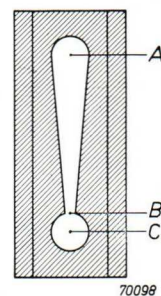
Fig. 96. Top view of the electrode system of the DM 70.
