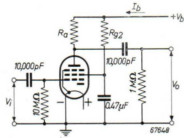
Fig. 33. Circuit diagram for the use of the pentode section as A.F. amplifier.
