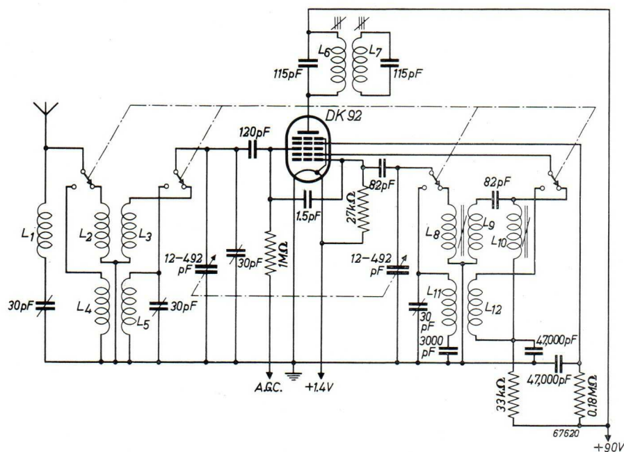
Fig. 3. Frequency changer circuit for the ranges 30 Mc/s to 9 Mc/s (10 m to 33 m) and 10 Mc/s to 3.3 Mc/s (30 m to 90 m). In the range 30 Mc/s to 9 Mc/s the A.G.C. should be switched off.
