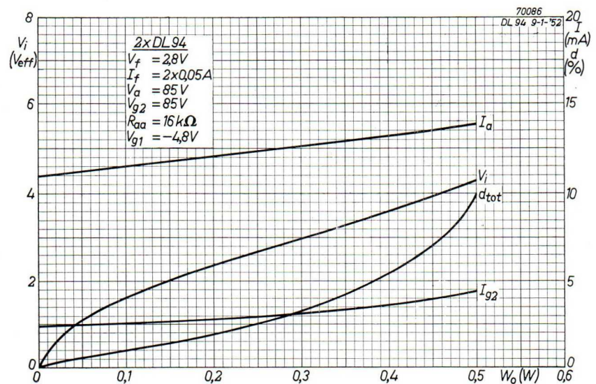
Fig. 84. Performance of two DL 94 tubes in push-pull class A for V_b = 90 V and V_f = 2.8 V, I_f = 2 \times 0.05 A (filament sections of each tube in series, filaments of the two tubes together in parallel).
