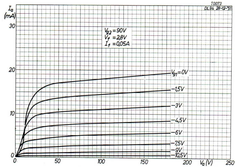
Fig. 71. Anode current plotted against anode voltage for V_{g2} = 90 V and V_f = 2.8 V, I_f = 0.05 A.
