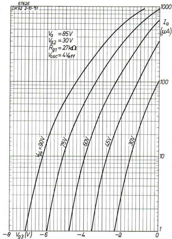
Fig. 9. Anode current as a function of the third-grid voltage with the screen-grid voltage as parameter, for V_a = 85 V.
