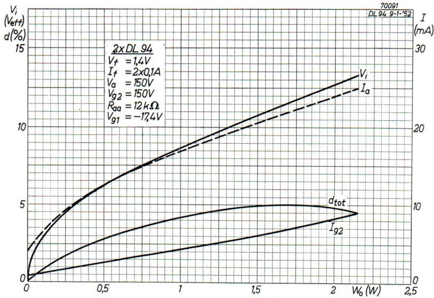
Fig. 89. Performance of two DL 94 tubes in push-pull class B for V_b = 150 V and V_f = 1.4 V, I_f = 2 \times 0.1 A (all filament sections in parallel).
