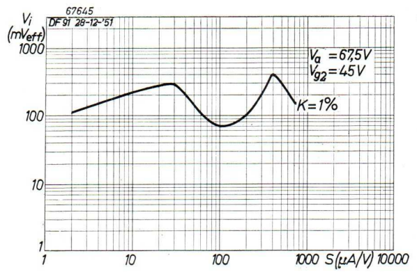
Fig. 29. Input signal plotted against the mutual conductance for a cross modulation of 1%, for V_a = 67.5\text{ V} and V_{g2} = 45\text{ V} .
