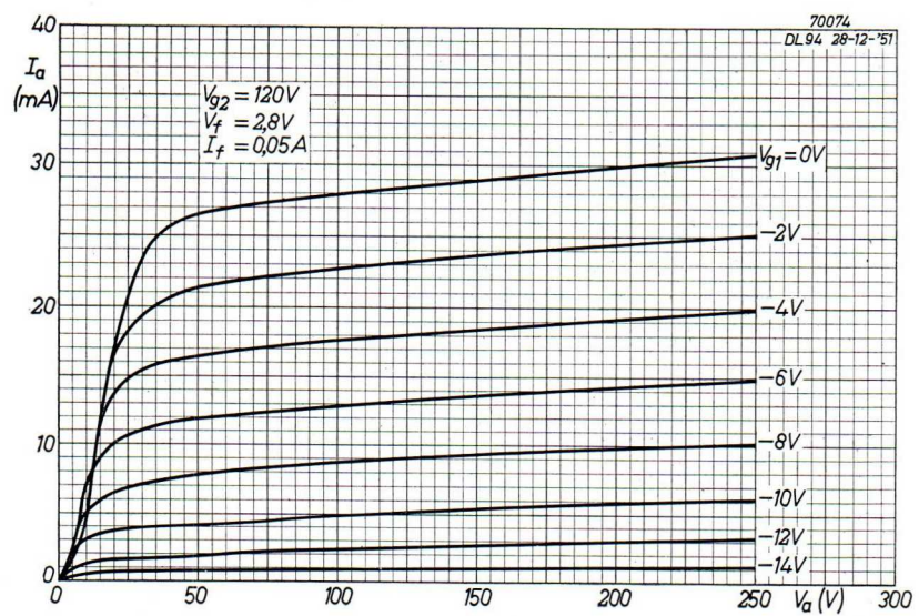
Fig. 72. Anode current plotted against anode voltage for V_{g2} = 120 V and V_f = 2.8 V, I_f = 0.05 A.
