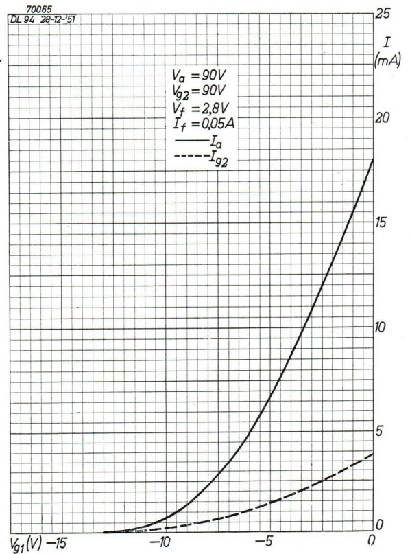
Fig. 63. Anode current and screen-grid current plotted against the control-grid voltage for V_a = V_{g2} = 90 V and V_f = 2.8 V, I_f = 0.05 A (two filament sections in series).
