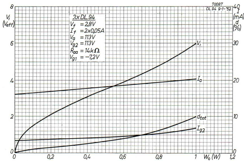
Fig. 85. Performance of two DL 94 tubes in push-pull class A for V_b = 120V and V_f = 2.8V , I_f = 2 \times 0.05A (filament sections of each tube in series, filaments of the two tubes in parallel).
