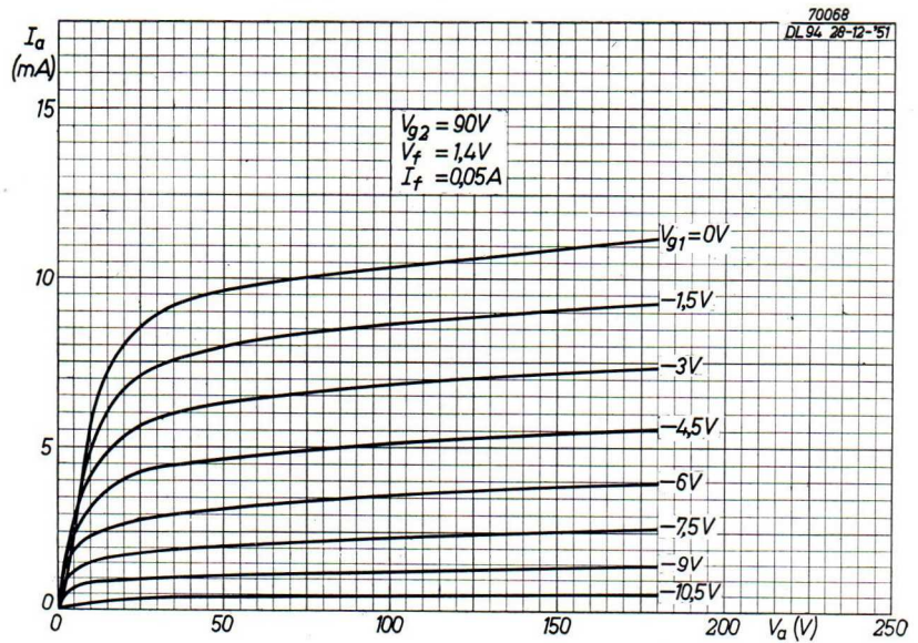
Fig. 66. Anode current plotted against anode voltage for V_{g2} = 90V and V_f = 1.4V , I_f = 0.05A .
